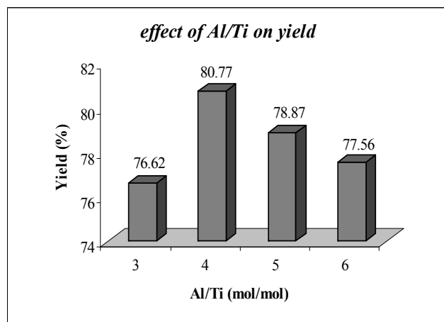
Fig. 5. The effect of Al/Ti on yield of reaction
