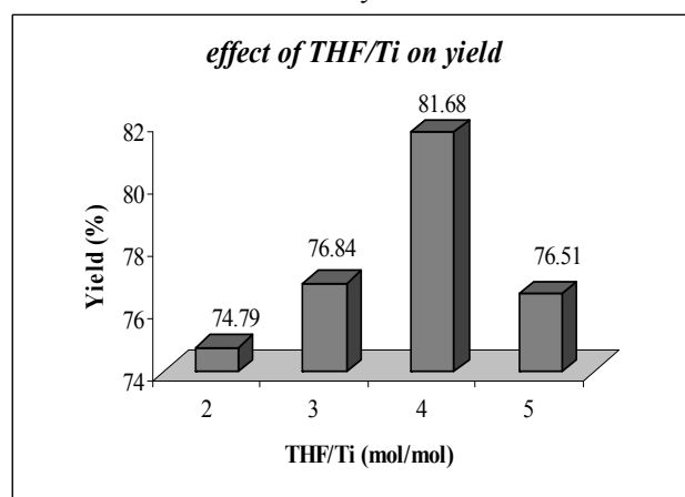
Fig. 6. The effect of THF/Ti on yield of reaction
