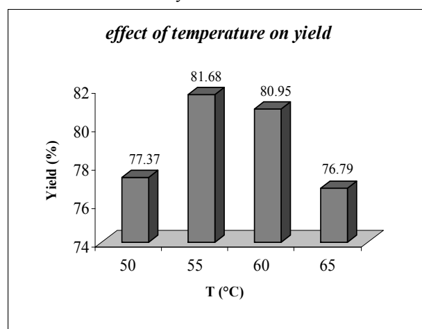
Fig. 3. The effect of reaction temperature on yield of reaction
