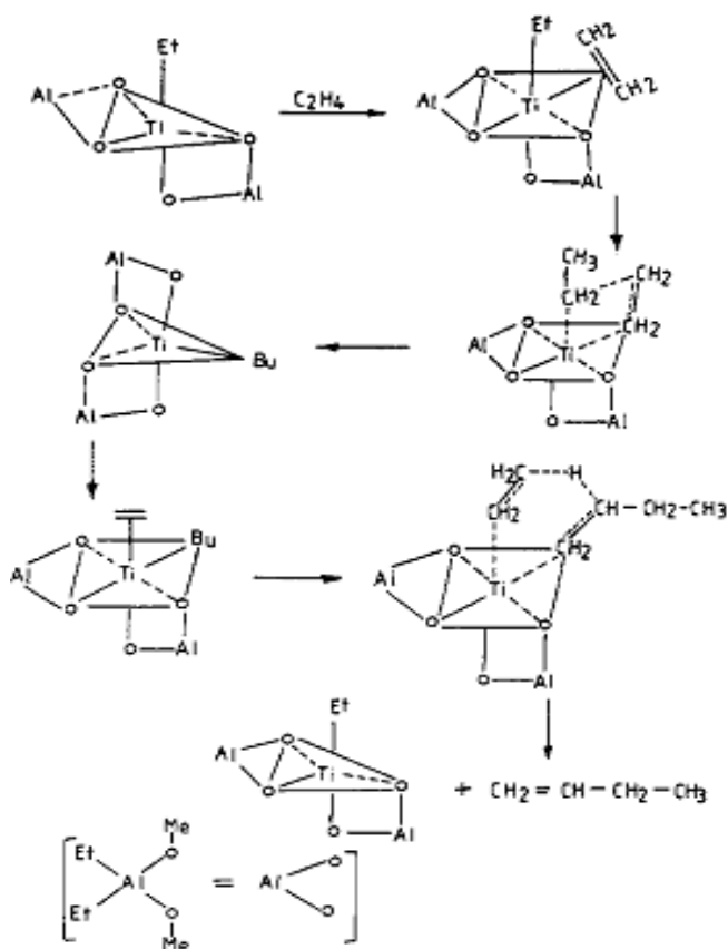
Fig. 1. A schematic representation for the bimetallic mechanism [6]
