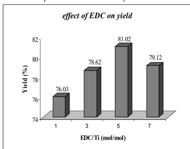
Fig. 7. The effect of EDC/Ti on yield of reaction
