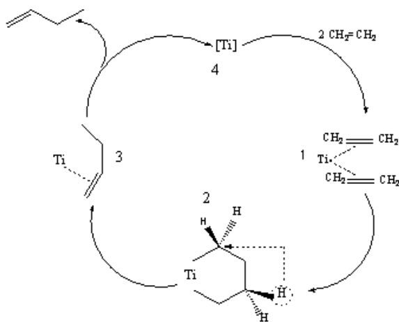
Fig. 2. Schematic representation of the cyclic intermediate mechanism
