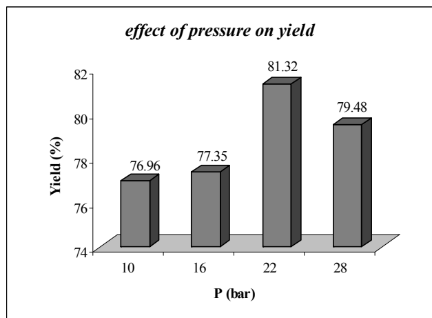
Fig. 4. The effect of reaction pressure on yield of reaction
